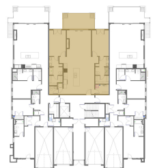
FLOOR PLAN
